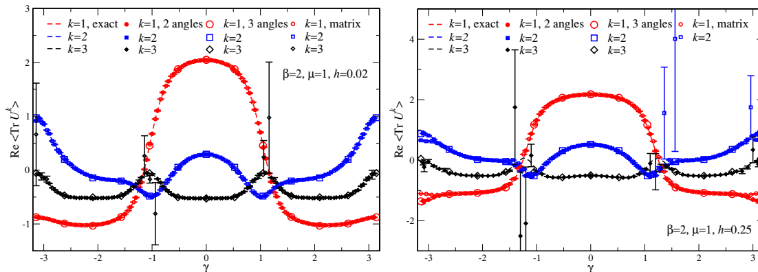
Figure 4. SU(3) one-link model: \langle \text{Tr } U^k \rangle vs. \gamma for k = 1, 2, 3 , at \beta_{\text{eff}} = 2, \mu = 1 and h = 0.02 (left) and 0.25 (right), using the two- and three-angle and the matrix formulations. At h = 0.02 , agreement with the exact results is seen for all \gamma in the two- and three-angle case; in the matrix case there is poor convergence at specific values of \gamma . At larger h = 0.25 , there is poor or wrong convergence also in the two- and three-angle case.
