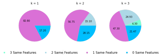
Figure 5. Comparing the shared features using SHAP and LIME.
