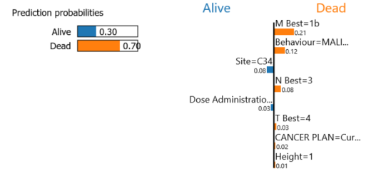
Figure 3. LIME providing an explanation given probability of Alive / Deceased cases. Supported by each feature value and importance towards the corresponding class of feature weighting.
