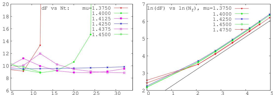
Figure 26. Left: difference \Delta F_{\text{eff}} between the free energy associated with the \text{Re } D < 0 region and the full one vs N_\tau . Right: \Delta F_{\text{eff}}(N_f) vs N_f for N_f flavours (double logarithmic scale). The straight line suggests a scaling \Delta F_{\text{eff}}(N_f) = \Delta F_{\text{eff}}(1)N_f^p with p \simeq 0.95 . Parameters are \beta = 0.25 , \kappa = 0.12 , ordered lattice, various \mu .
