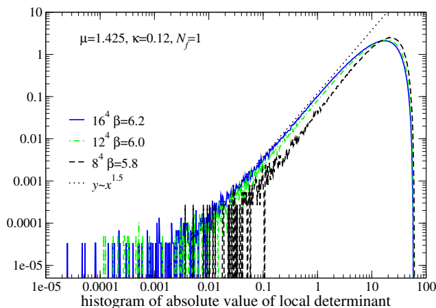
Figure 31. As in figure 28, with a decreasing lattice spacing ( \beta = 5.8, 6.0, 6.2 ), while keeping the physical volume approximately constant (with lattice volume 8^4, 12^4, 16^4 ), using \kappa = 0.12, \mu = 1.425, N_f = 1 .
