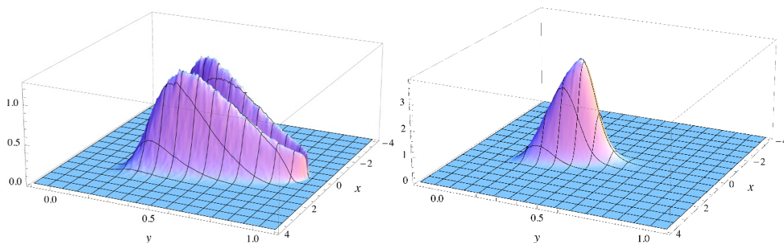
Figure 6. Histogram P(x, y) for z_p = i , n_p = 2 , \beta = 1.6 (left) and \beta = 3.2 (right).
