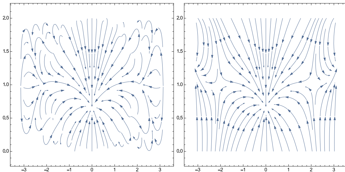
Figure 38. Flow pattern for the U(1) one-link model at \beta = 0.3 , n_p = 1 , \mu = 1 , \kappa = 2 , using the Taylor expansion to order N = 10 with D_0 = 1 + \kappa \cos(0.8i) (left) and the full expression (right).
