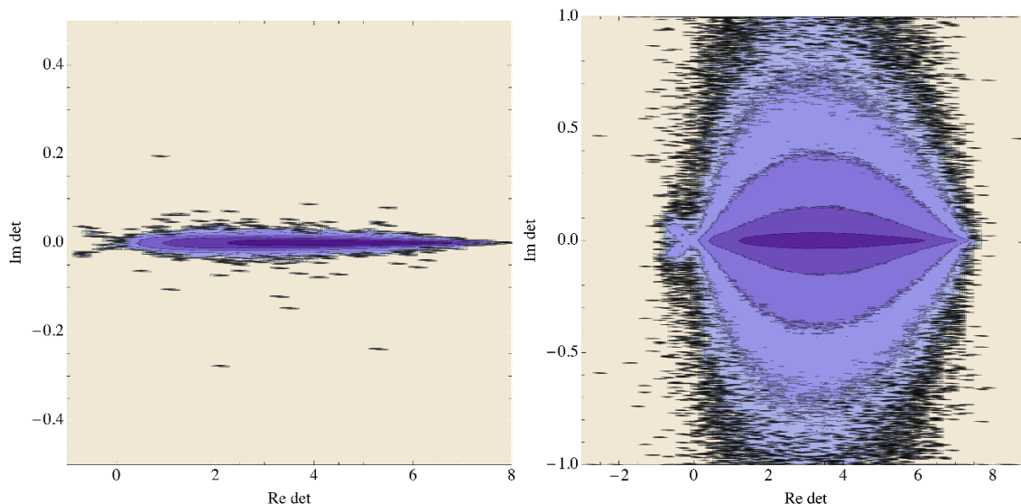
Figure 30. As in figure 29, on a 8^4 (left) and 16^4 (right) lattice at \beta = 5.9, \kappa = 0.12, \mu = 1.425, N_f = 1 . Note the different scale.
