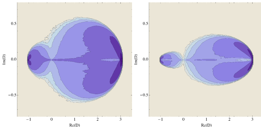
Figure 12. Logarithmic contour plots of the distribution of the complex determinant D , for \beta = 0.3, \kappa = 2, \mu = 1, n_p = 1 (left) and n_p = 2 (right).
