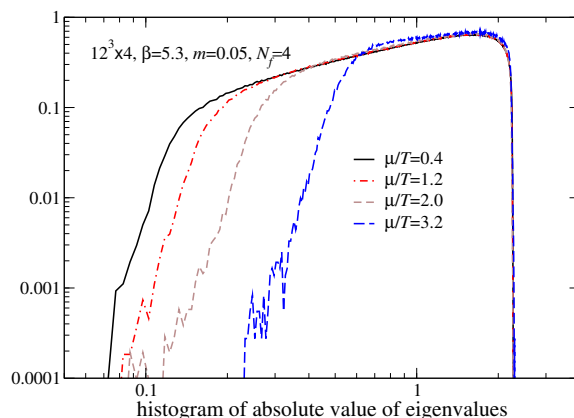
Figure 35. Histogram of the absolute value of eigenvalues for full QCD, gained averaging the spectrum from 100 configurations.
