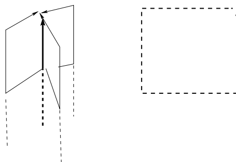
Figure 15. Effective one-link model for the Polyakov line in temporal gauge in the field of its neighbours.
