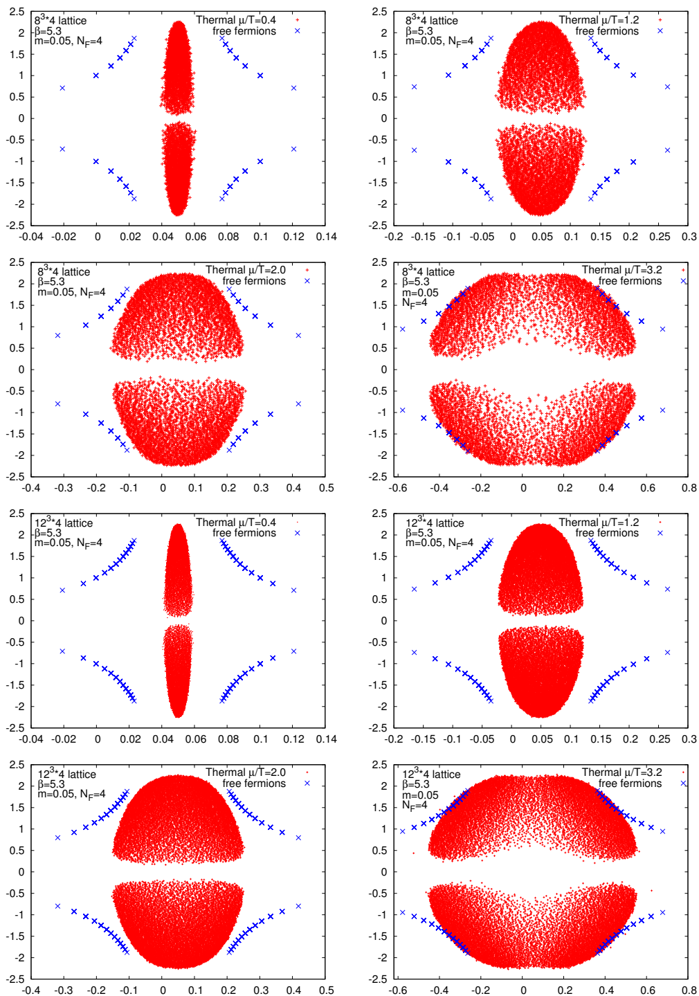
Figure 34. Spectrum of the staggered fermion operator on a 8^3 \times 4 lattice (top four panels) and 12^3 \times 4 lattice (bottom four panels), for \mu/T = 0.4, 1.2, 2.0, 3.2 . The free spectrum is shown as well. Other parameters as in figure 32.
