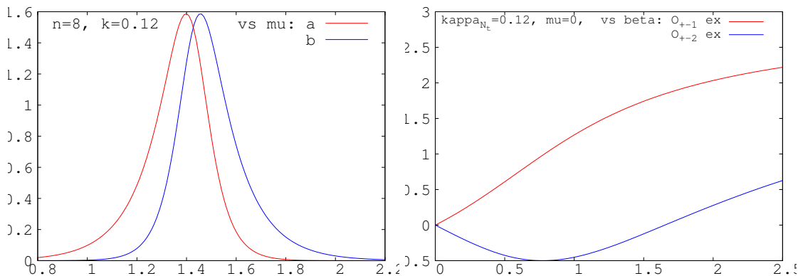
Figure 16. Left: coefficients a, b vs \mu for N_\tau = 8, \kappa = 0.12 . Right: observables \langle O_{\pm 1} \rangle, \langle O_{\pm 2} \rangle vs \beta at N_\tau = 8, \kappa = 0.12, \mu = 0 .
