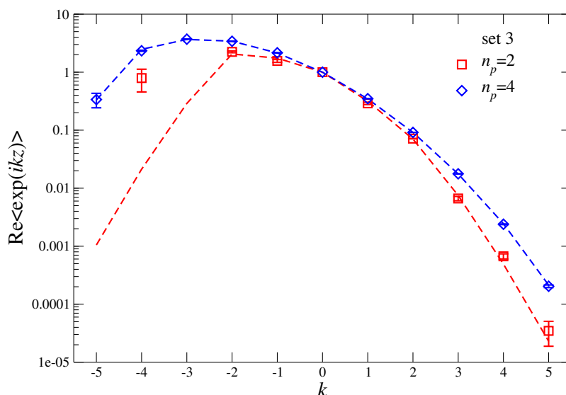
Figure 14. \text{Re}\langle \exp ikz \rangle for k = -5, \dots, 5 vs k , on a logarithmic scale, for parameter set (3), with n_p = 2, 4 . The lines are the exact results.
