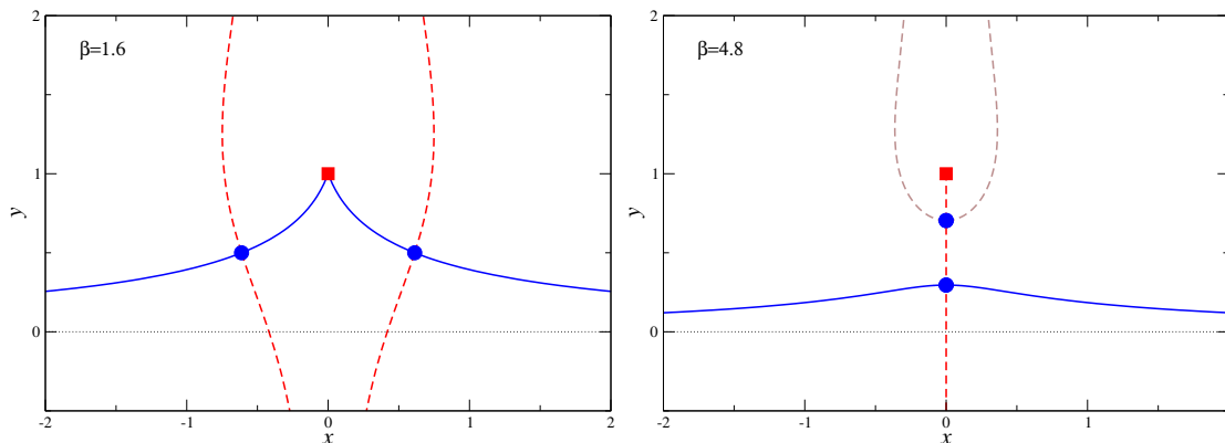
Figure 4. Thimbles corresponding to figure 3. See text for details.
