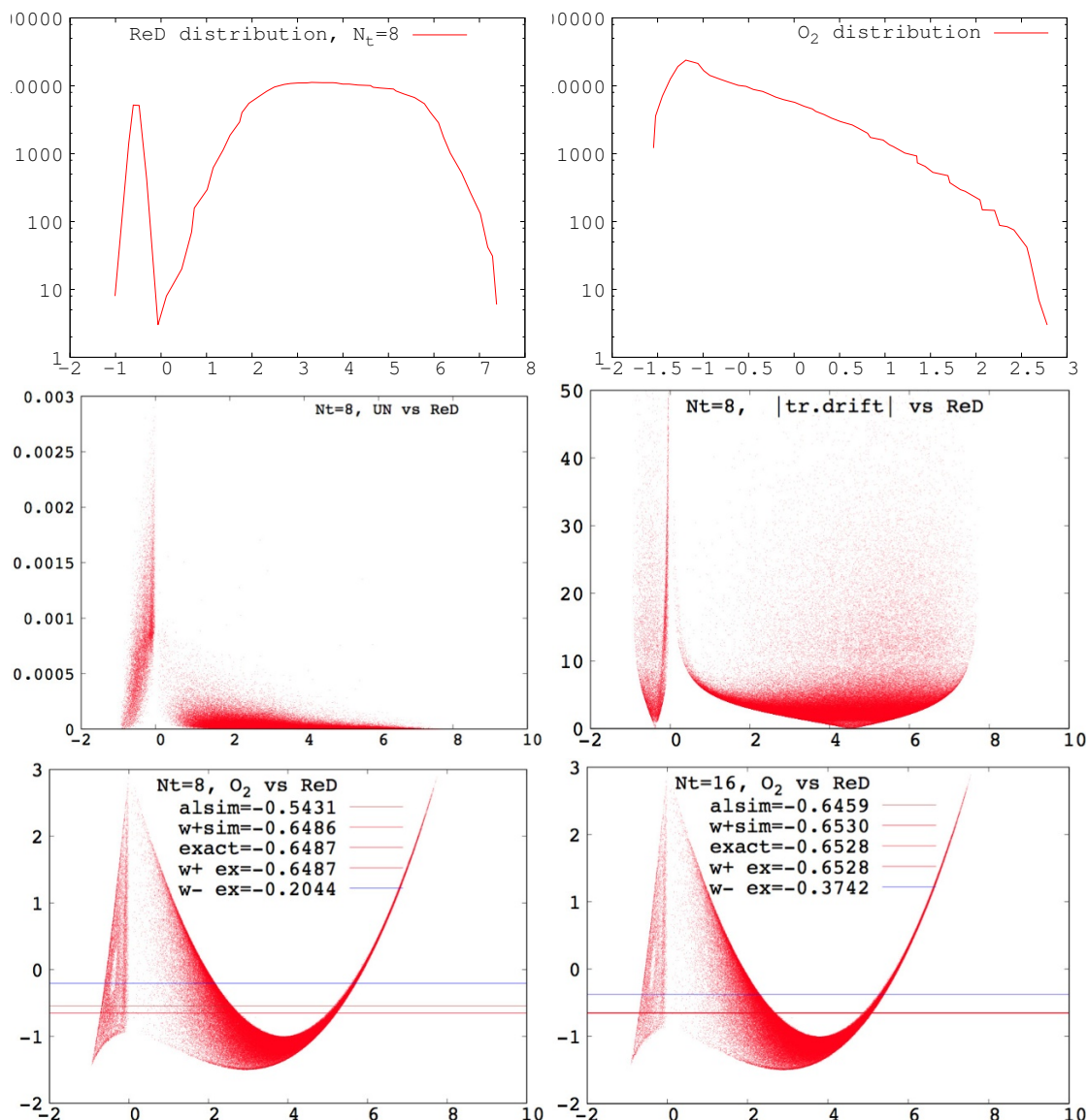
Figure 21. Top: histograms of \text{Re } D (left) and O_2 = \text{tr } U^2 (right). Middle: correlation between \text{Re } D and the unitarity norm \text{tr}(U^\dagger U - \mathbb{1}) (left), and between \text{Re } D and the norm of the instantaneous drift force. Bottom: correlation between \text{Re } D and O_2 for N_t = 8 (left) and 16 (right). Parameters as above, with \mu = 1.425 .
