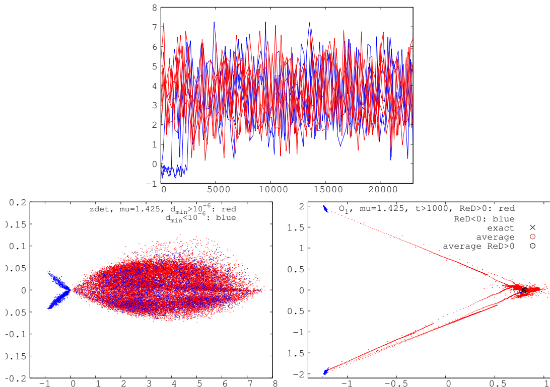
Figure 22. As in figure 19 for the strongly disordered lattice
