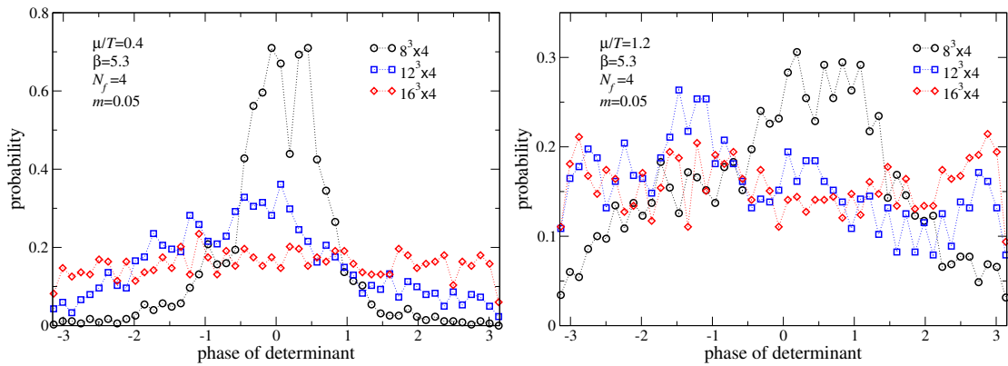
Figure 33. Histogram of the phase of the determinant for three spatial volumes for \mu/T = 0.4 (left) and \mu/T = 1.2 (right). Other parameters as in figure 32.
